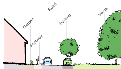
Typical tertiary fringe
