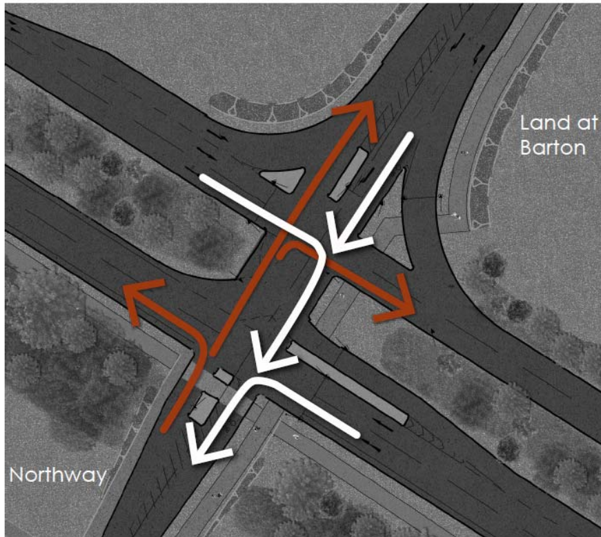
Illustration 9: Potential bus and emergency vehicle movements to/from Northway
